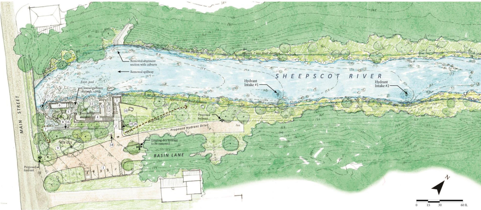
Coopers Mills - Conceptual Site Design Alternative B
